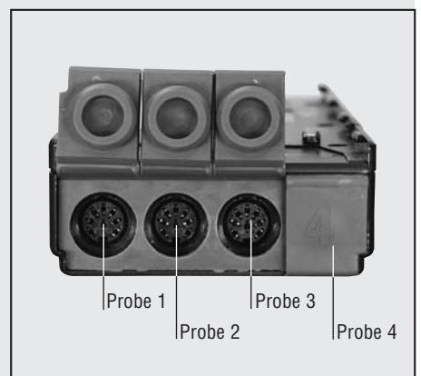
Connections 1: Probe
