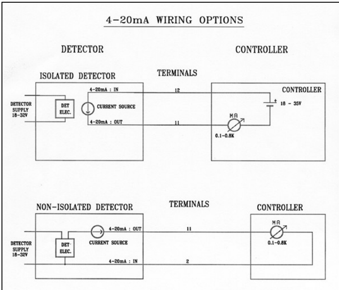
Figure 16: 4-20mA wiring
