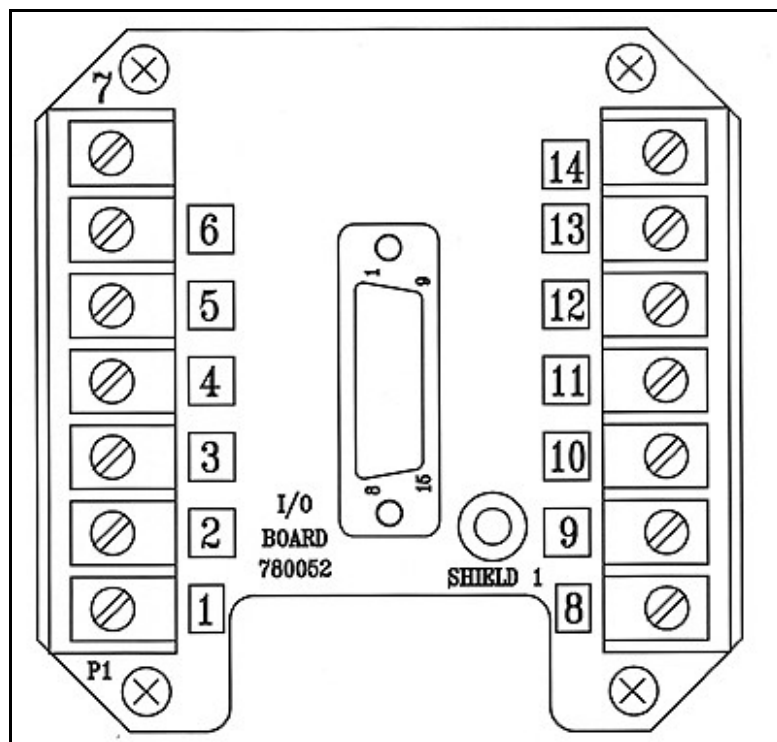
Figure 10: Terminal Board
