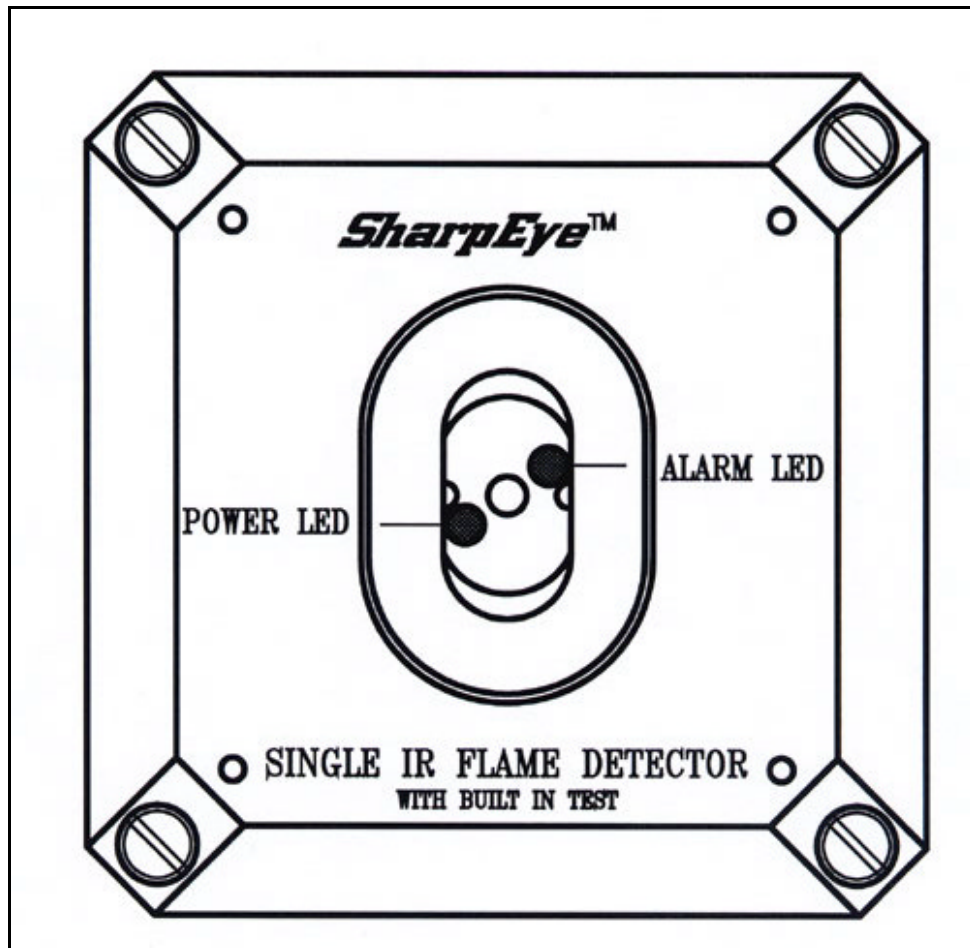
Figure 4: Indication LEDs
